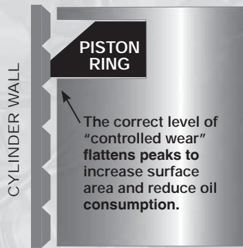
Fig. 2: Broken-In Cylinder
